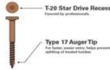
Cap Top w/ Epoxy Coated Carbon Steel 100 pcs/30 sq ft
